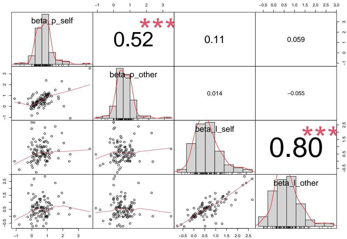
Appendix Figure C2. correlation of the coefficients from Grether's model estimated individually. This includes only the HP.
