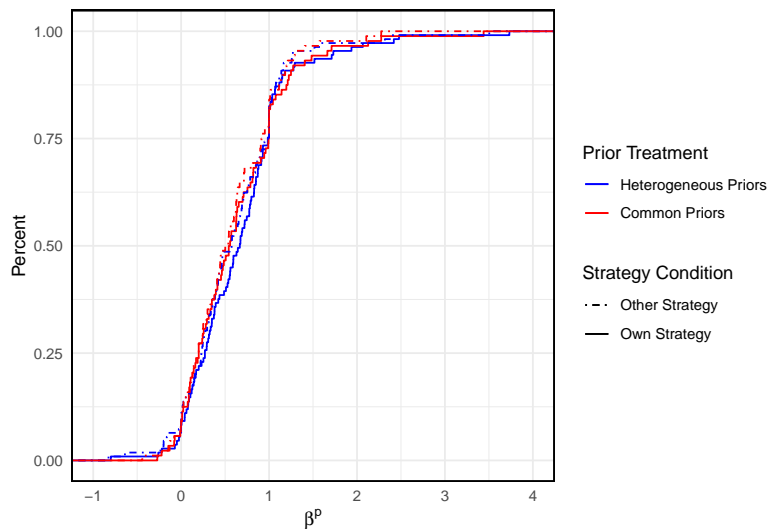
Figure 10. Distribution of \beta^p by treatment. Difference between the second prior and first order prior based on the CP condition. Sensitiveness of the bias to the signal.
